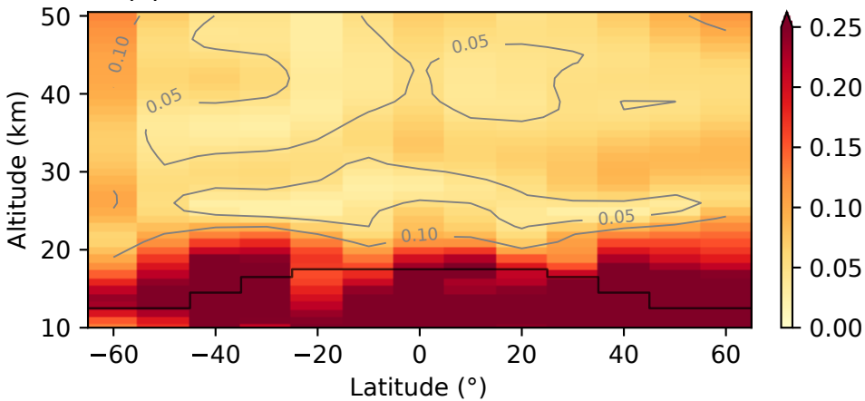
(c) Normalized ozone standard deviation
