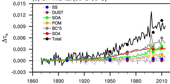
(e) SH Mid-lat (30°S-60°S)
