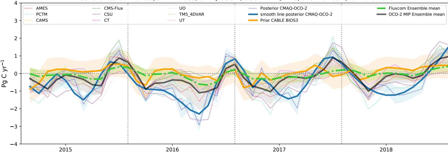
Australian carbon fluxes (CABLE BIOS3, CMAQ-OCO-2, OCO-2 MIP (LNLG) and FLUXCOM) for 2015-2018
