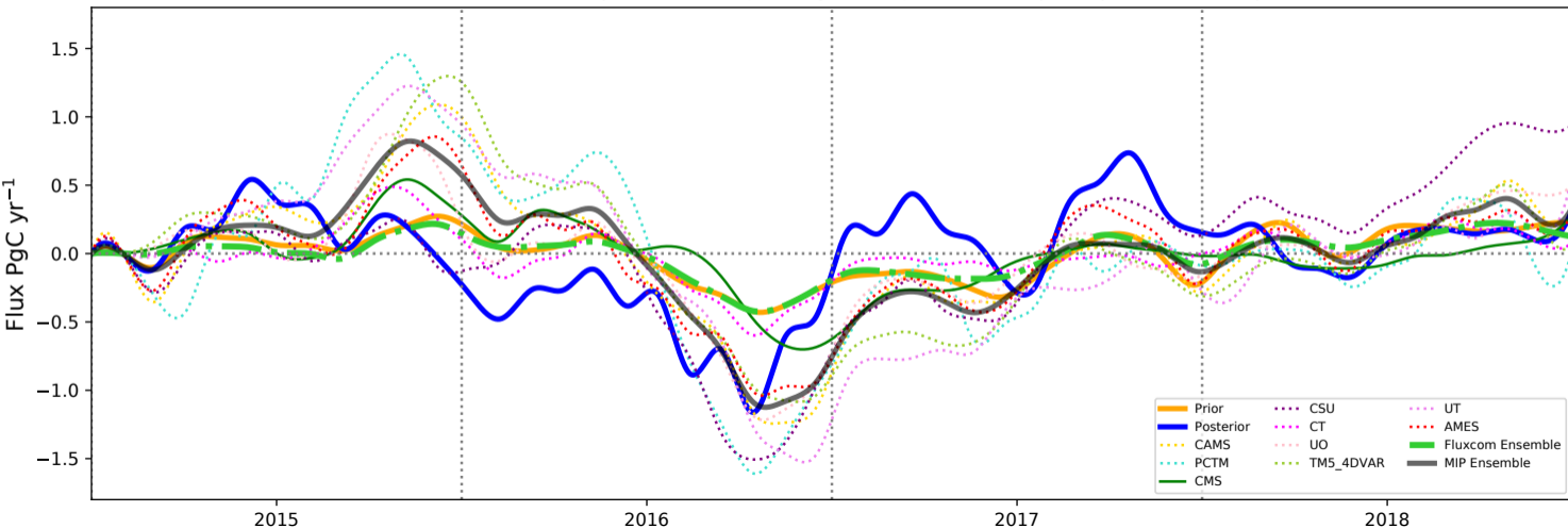
Australian carbon flux anomalies (CABLE BIOS3, CMAQ-OCO-2, OCO-2 MIP (LNLG) and FluxCom) for 2015-2018
