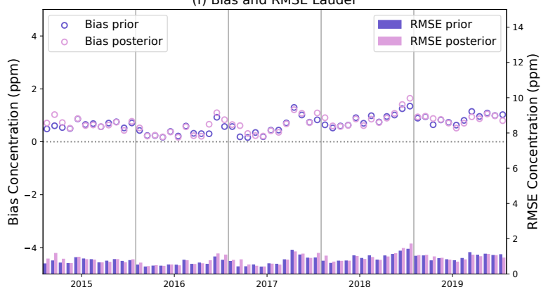
(f) Bias and RMSE Lauder
