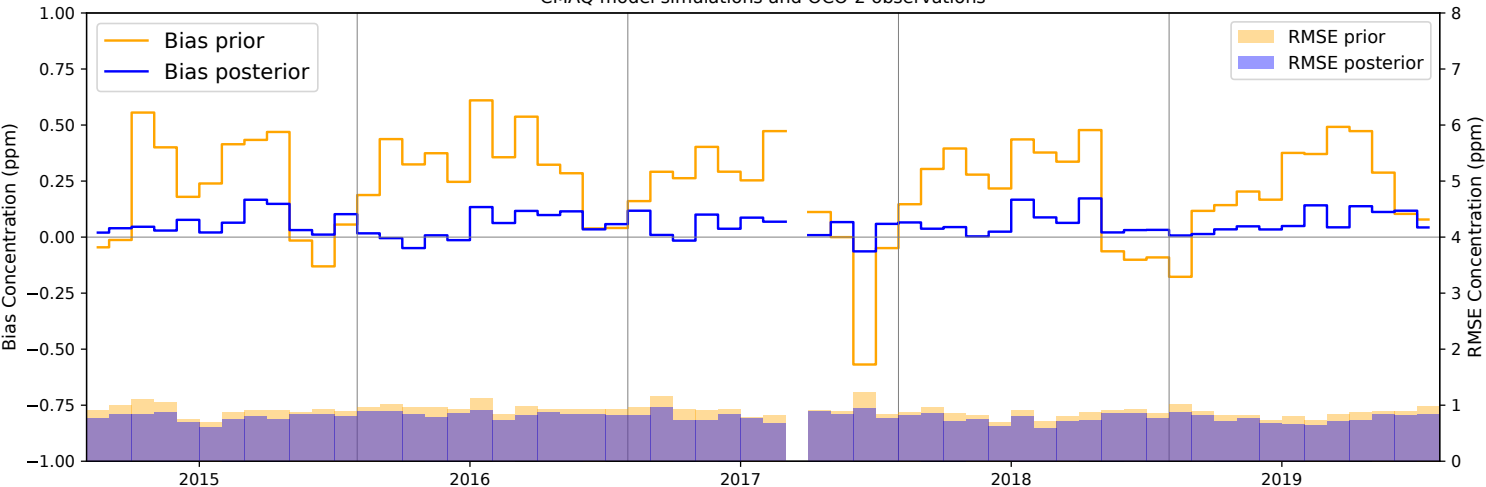
CMAQ model simulations and OCO-2 observations
