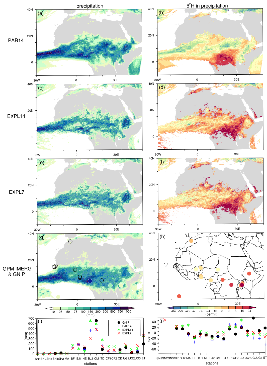
Figure S1. As Fig. 3, but for June 2016.
