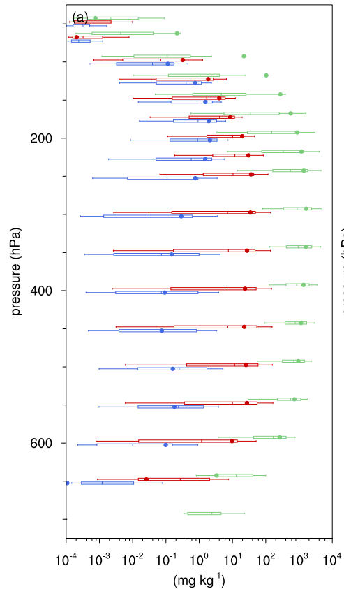
ice content
