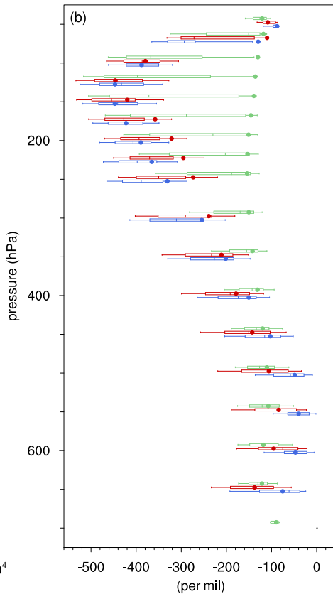
\delta^2\text{H}_{\text{ice}}
