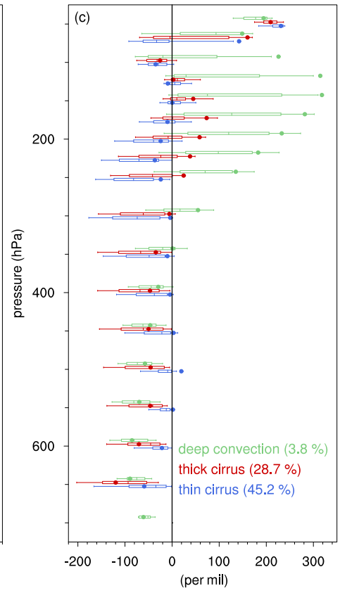
\delta^2\text{H}_{\text{ice}}
