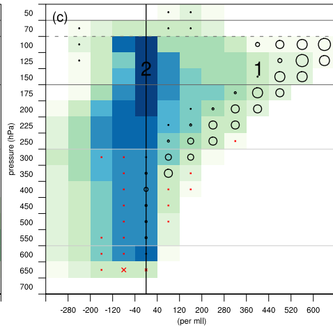
disequilibrium in ice ( \delta^2\text{H}_{\text{Ice}} - \delta^2\text{H}_{\text{Ice,eq}} )
