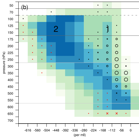
\delta^2\text{H}_{\text{Ice}}
