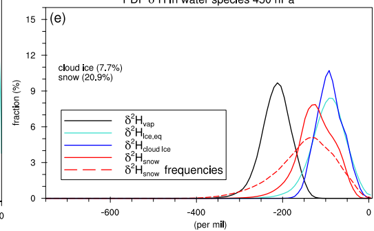
PDF \delta^2\text{H} in water species 450 hPa
