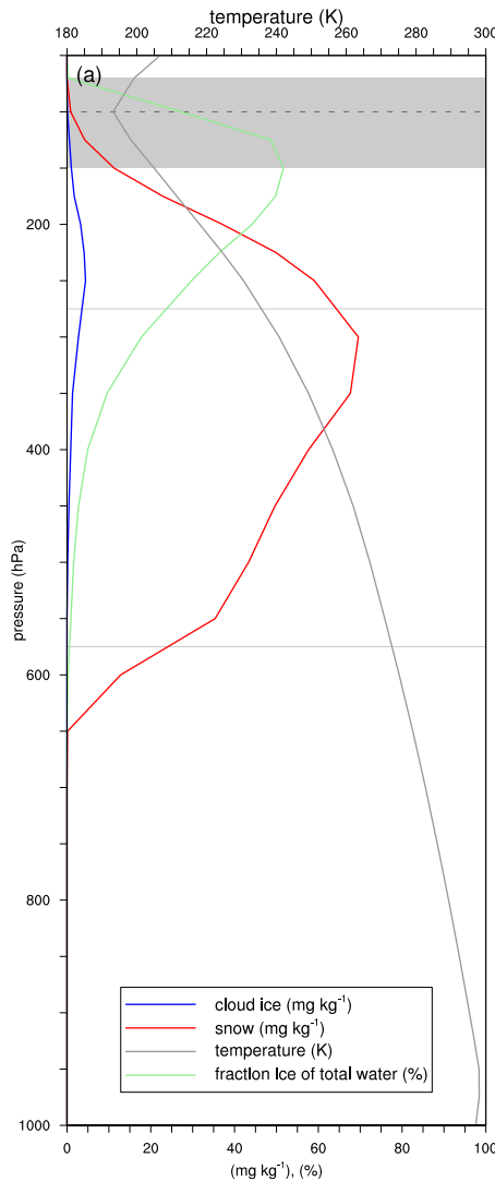
vertical profiles of water species
