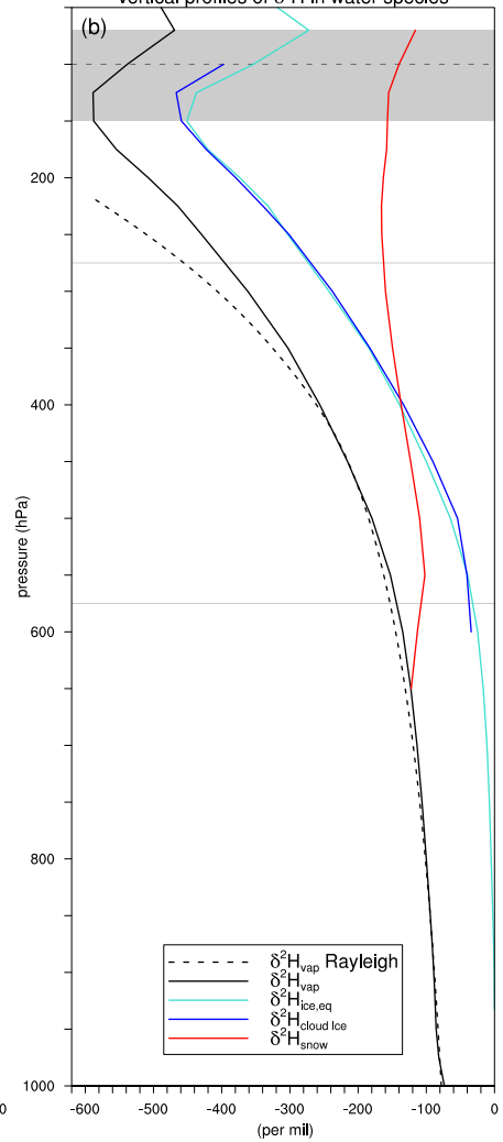
vertical profiles of \delta^2\text{H} in water species
