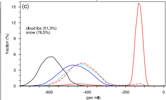
PDF \delta^2\text{H} in water species 200 hPa
