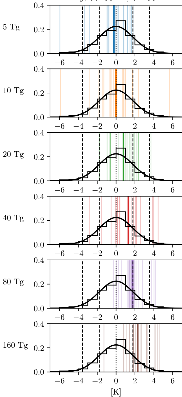
\Delta'T_s, 50-80^\circ\text{N}, 0-150^\circ\text{E}
