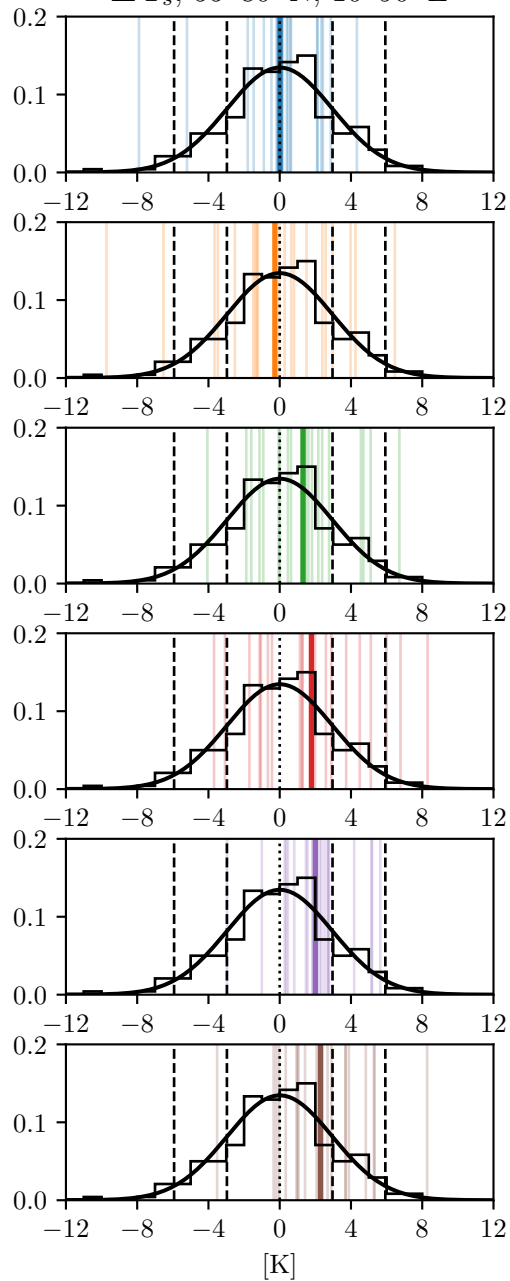
\Delta'T_s, 55-80^\circ\text{N}, 10-90^\circ\text{E}
