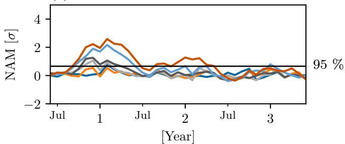
(c) 850 hPa
