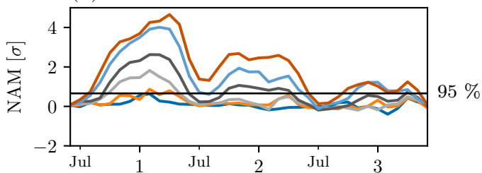
(c) 850 hPa
