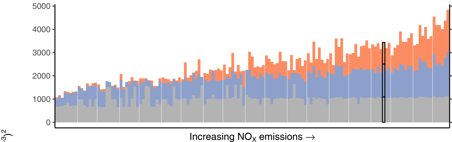
(b) Median MSE in MDA8 \text{O}_3 concentrations
