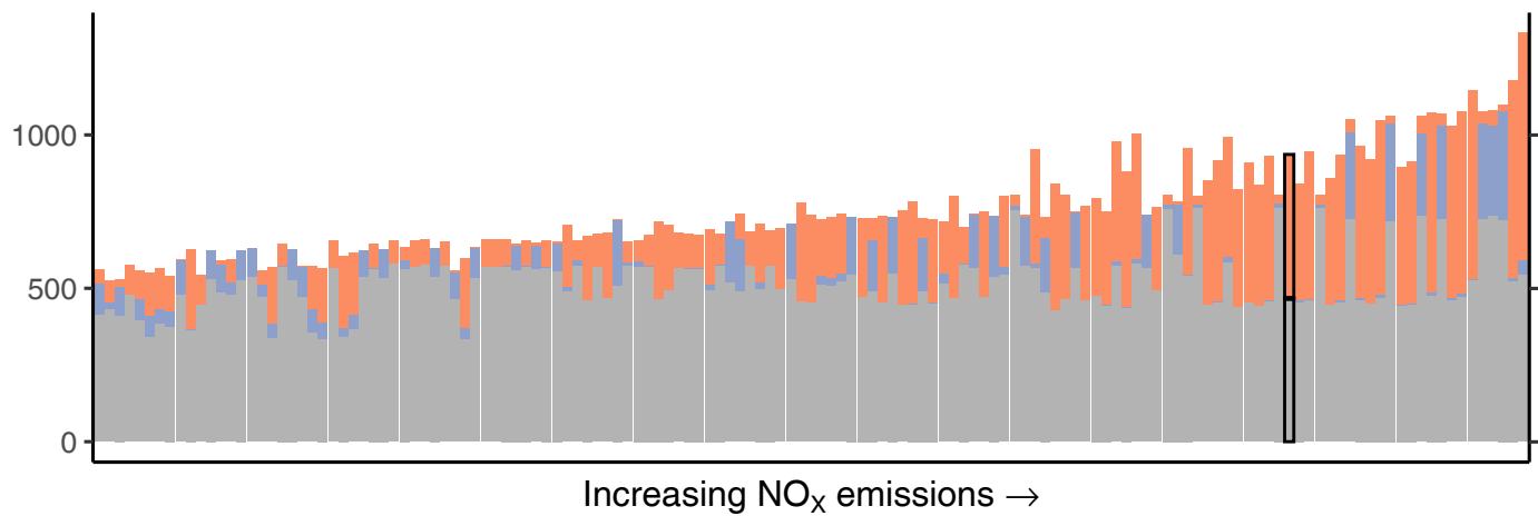
(b) Median MSE in MDA8 \text{O}_3 concentrations
