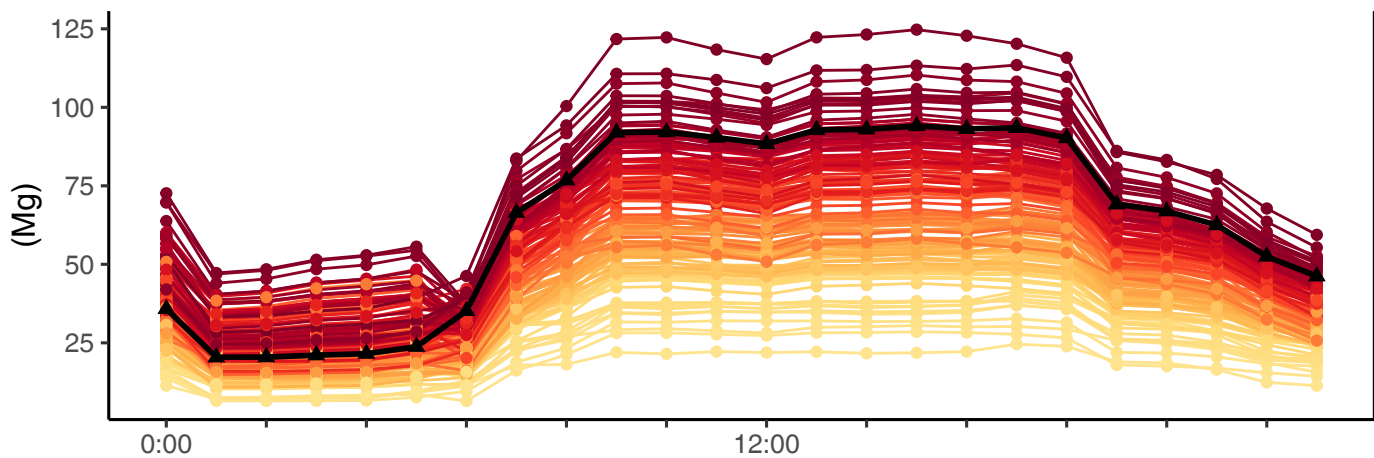
(c) Mean diurnal variations in total \text{NO}_x emissions
