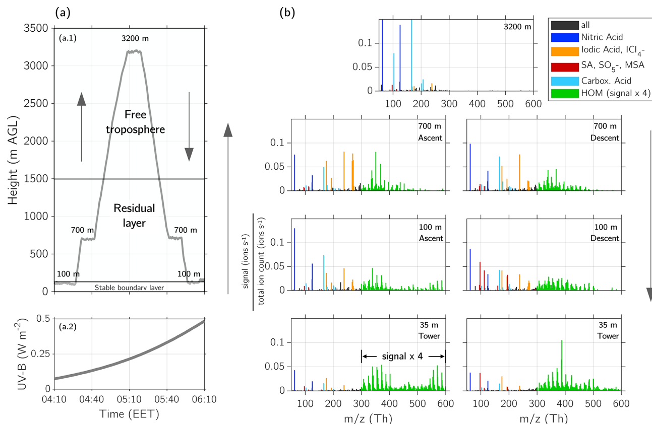
Figure 6. Vertical profile of ions above Hyytiälä on 2 May 2017 at 04:00–06:00 EET. (a.1) Height profile of the flight measurements and indication of the different layers (stable boundary layer (SBL), residual layer (RL), and free troposphere (FT)). (a.2) UV-B radiation measured on the ground at SMEAR II station during the flight. (b) Mass spectra measured with API-TOF at different heights. The altitude where the mass spectra were measured is indicated in the figures and can be compared with the height profile of panel (a). The lowest mass spectra show the measurements from the tower at SMEAR II station at 35 m height, while the presented data are covering the time period of the lowest level measurements at 100 m (04:10–04:20 and 05:55–06:05 EET) to be comparable. The signal of the HOM-dominated ions (green) between 300–600 Th is multiplied by a factor of 4 to make the pattern more visible. A peak list of the different layers can be found in Table A1. The colour code shows the composition of the compounds: nitric acid (blue), iodic acid and iodine–chlorine (yellow), sulfuric acid (SA), \text{SO}_5^- and MSA (red), carboxylic acids (cyan), and HOM-dominated ions (green).
