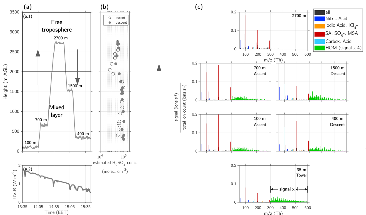
Figure 7. Vertical profile of ions above Hyytiälä on 2 May 2017 at 13:30–15:30 EET. (a.1) Height profile of the flight measurements and indication of the different layers (mixing layer (ML) and free troposphere (FT)). (a.2) UV-B radiation measured on the ground at SMEAR II station during the flight. (b) Estimated sulfuric acid concentration in molecules \text{cm}^{-3} during ascent (13:15–14:40 EET) and descent (14:40–15:30 EET), calculated based on Beck et al. (2022). (c) Mass spectra measured with API-TOF at different heights. The altitudes at which the mass spectra were measured are indicated in the figures and can be compared with the height profile of panel (a). The lowest mass spectrum shows the measurements from the tower at SMEAR II station at 35 m height. The presented data are an average from 14:00–16:00 EET. The signal of the HOM-dominated ions (green) between 300–600 Th is multiplied by a factor of 4 to make the pattern more visible. A peak list of the ML and the FT can be found in Table A1. The legend shows the colouring for compounds containing nitric acid (blue), iodic acid and iodine–chlorine (yellow), sulfuric acid (SA), \text{SO}_5^- and methanesulfonic acid (MSA) (red), carboxylic acids (cyan), and HOM-dominated ions (green).
