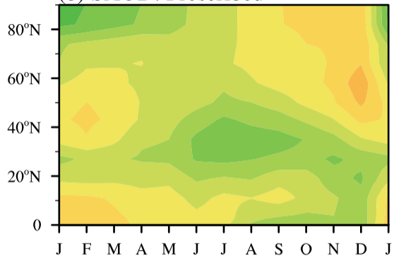
(b) SAOD: Prescribed
