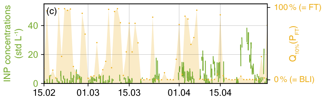
BG INP concentrations and air masses at the JFJ
