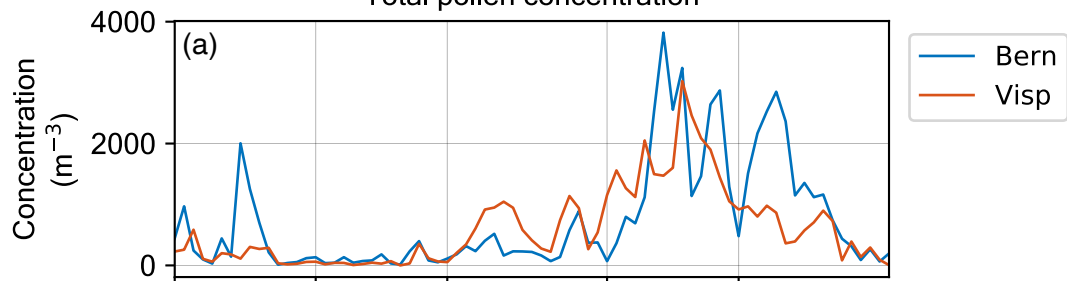
Birch, pine, cypress and grasses pollen
