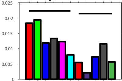
(a) \beta(\text{H}_2\text{O}_e, \text{QBO}) [ppmv (m/s) -1 ]
