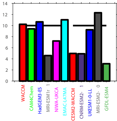
(b) SD of QBO 50hPa [m/s]
