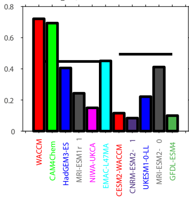
(c) r(\text{H}_2\text{O}_e, \text{QBO})
