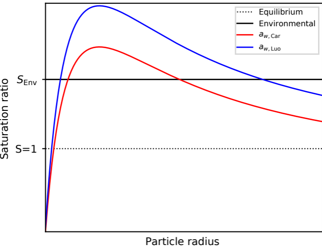
Schematical Koehler curves a_{w, Car} < a_{w, Luo}
