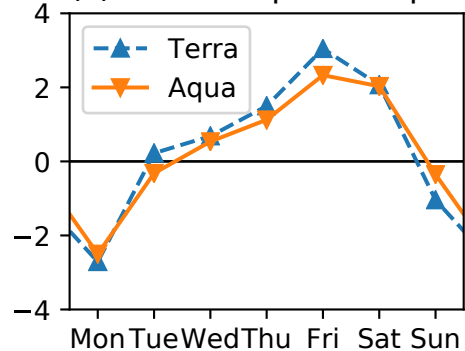
(c) Aerosol optical depth
