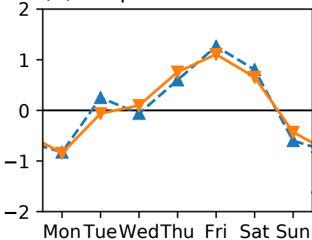
(b) Droplet number
