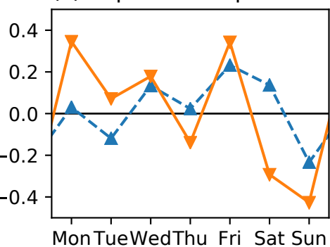
(c) Liquid water path
