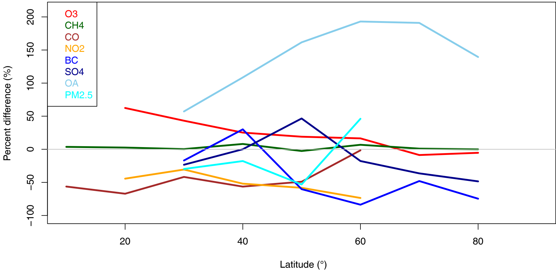
Change in mmm bias with latitude
