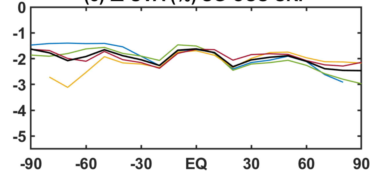
(c) \Delta UVA (%) SG-COS-SRF
