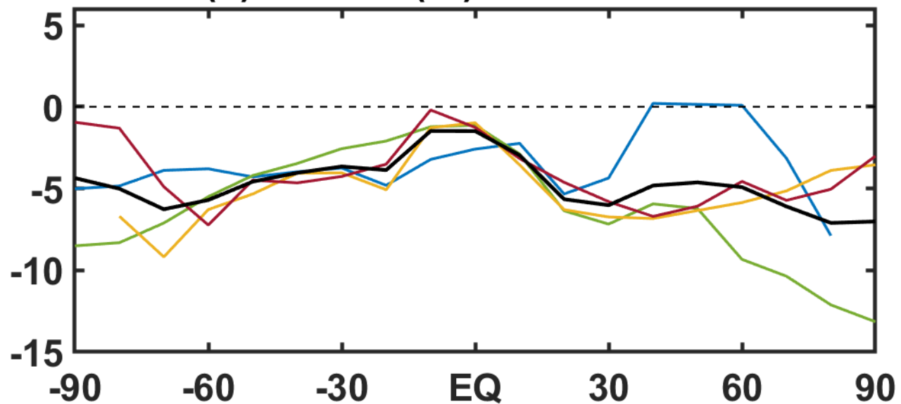
(a) \Delta UVB (%) SG-COS-SRF
