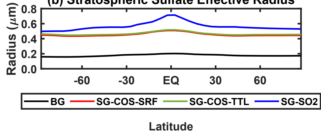
(b) Stratospheric Sulfate Effective Radius
