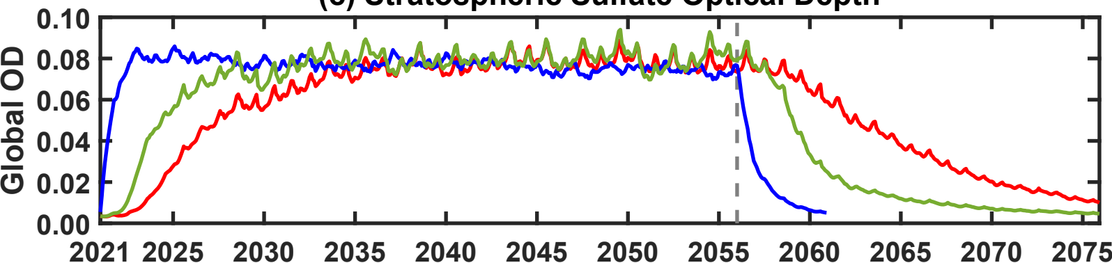
(c) Stratospheric Sulfate Optical Depth
