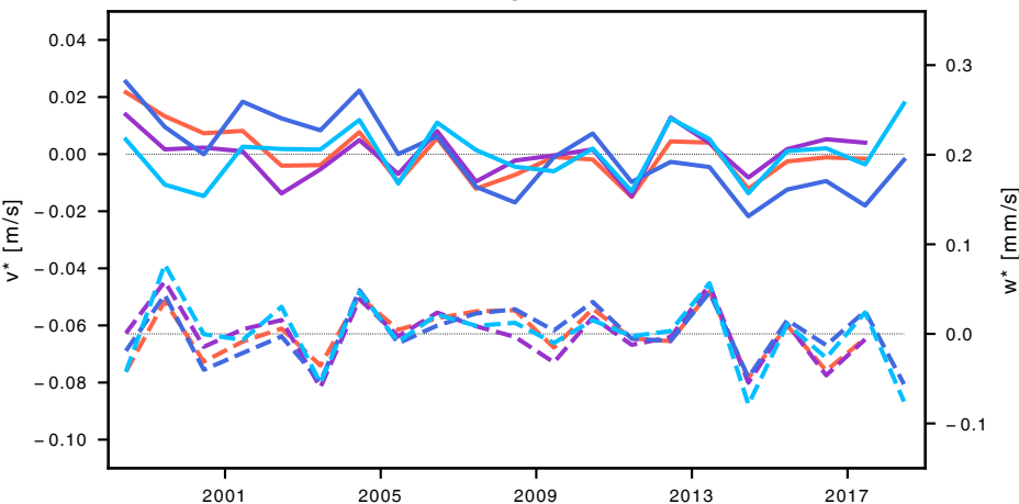
(a) Outflow & downwelling (NH)
