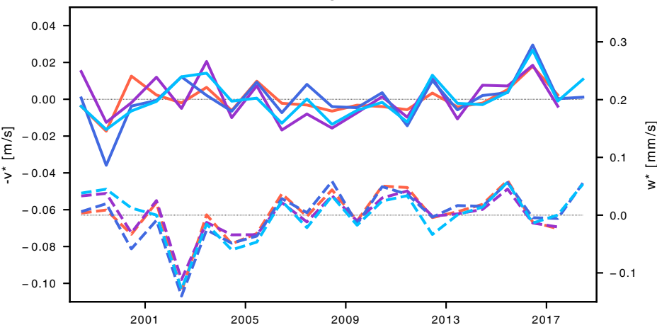
(b) Outflow & downwelling (SH)
