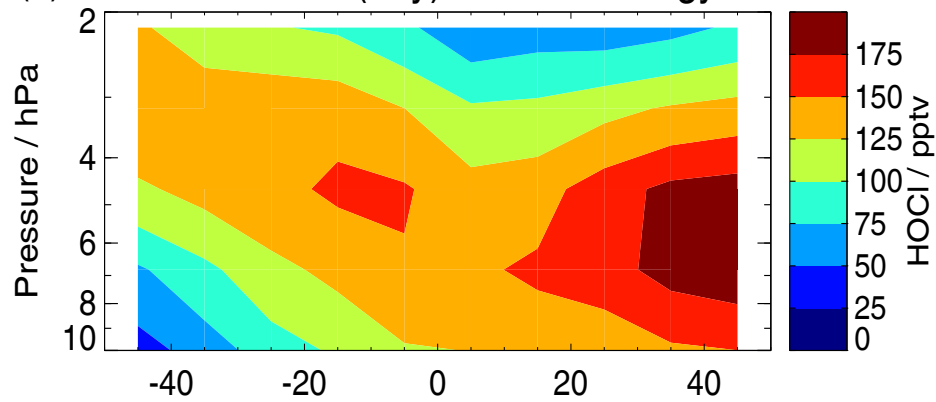
(e) Model HOCl (day) Jul Climatology
