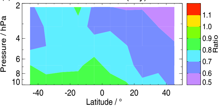
(c) Ratio Model/MLS HOCl (day) for Jan
