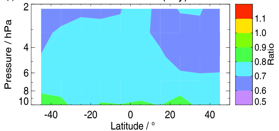
(f) Ratio Model/MLS HOCl (day) for Jul
