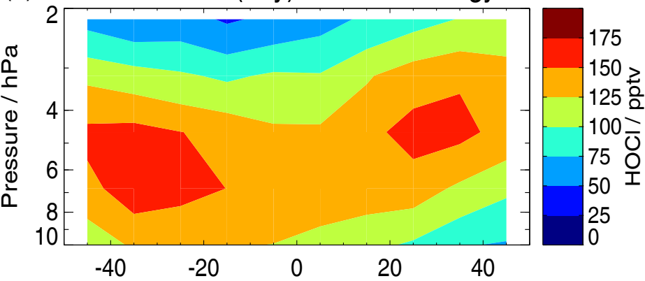
(b) Model HOCl (day) Jan Climatology
