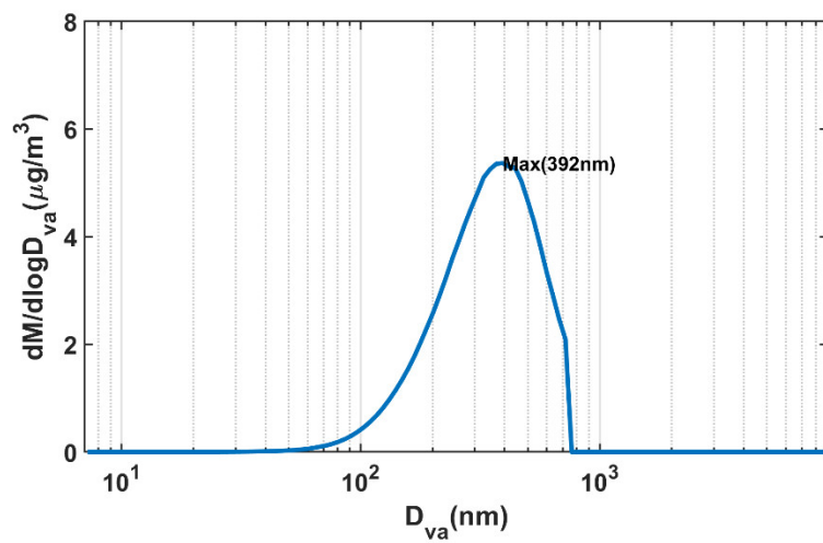
Figure S1: Particle mass size distributions.
