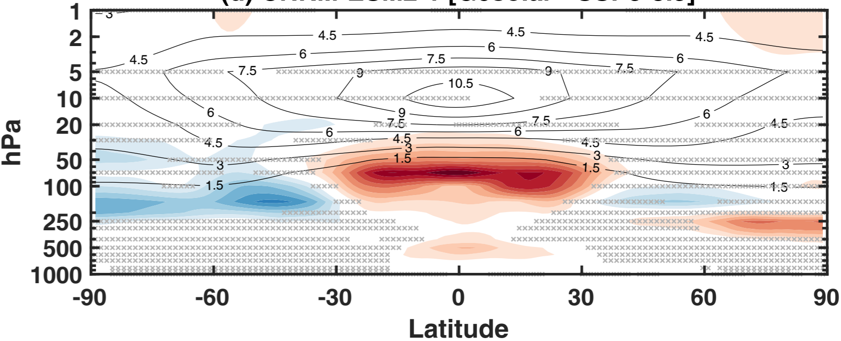
(f) UKESM1-0-LL [G6solar - SSP5-8.5]
