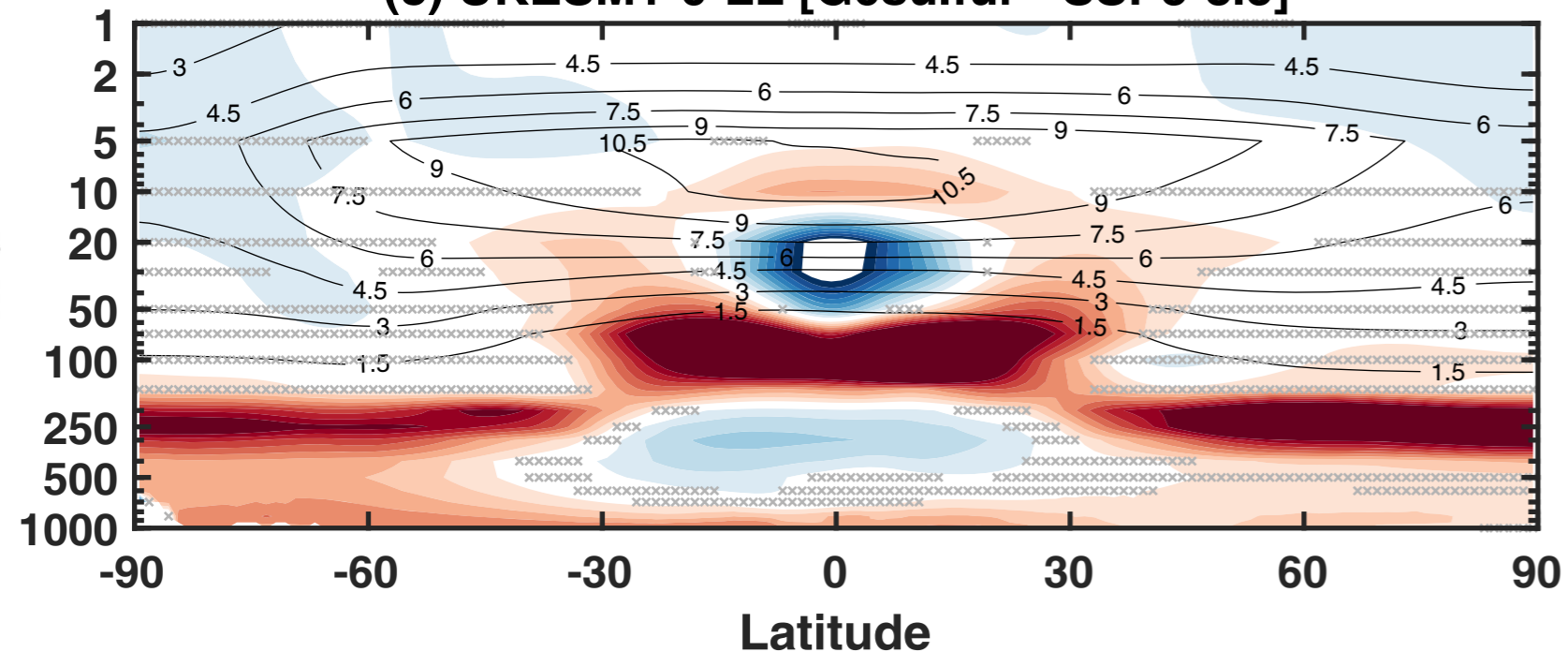
(e) UKESM1-0-LL [G6sulfur - SSP5-8.5]
