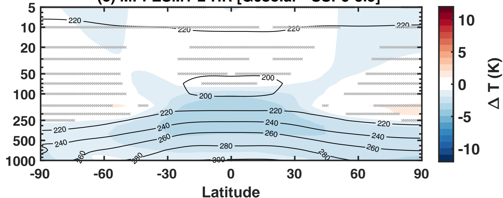
(e) MPI-ESM1-2-HR [G6solar - SSP5-8.5]
