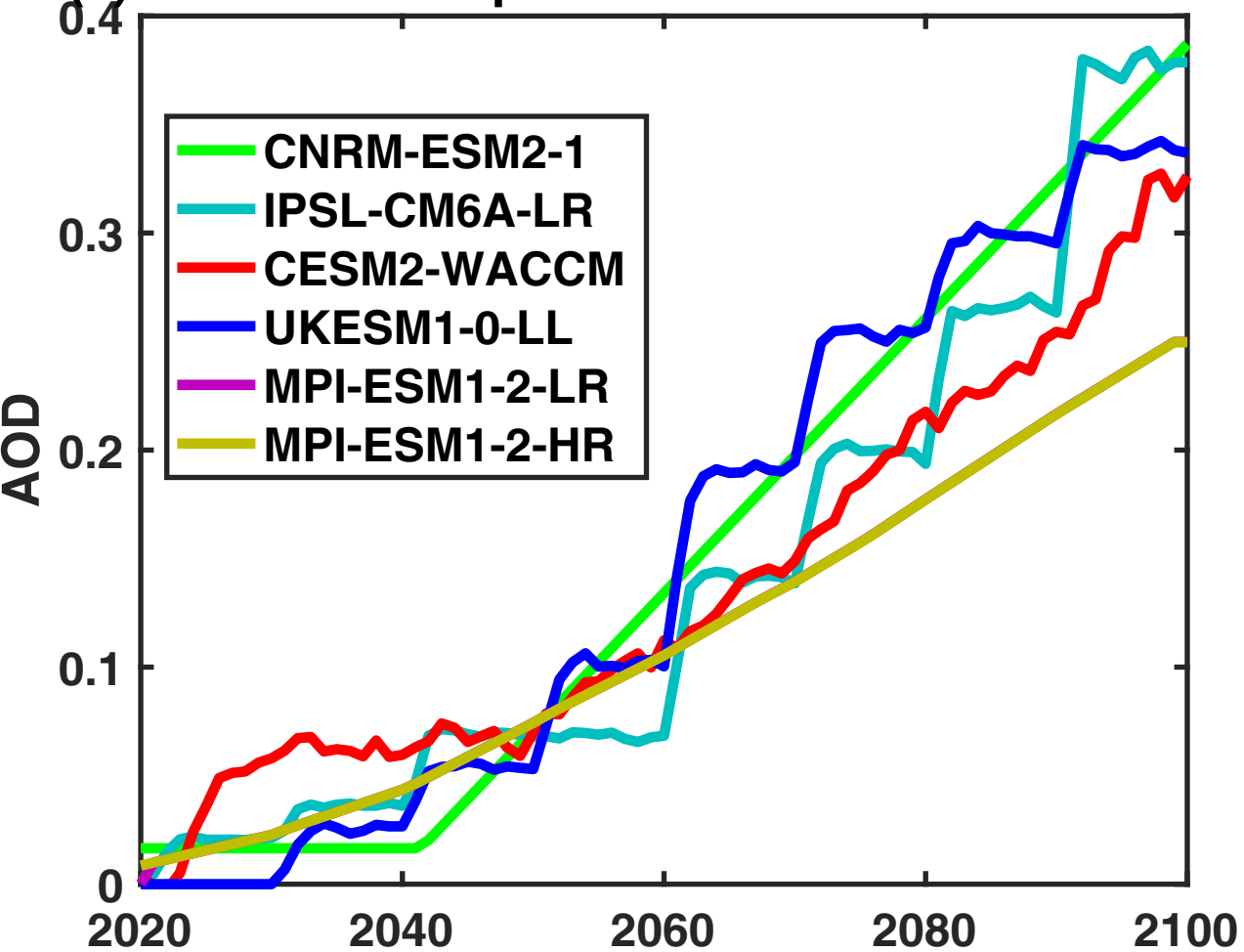
(a) Global stratospheric AOD increase in G6sulfur
