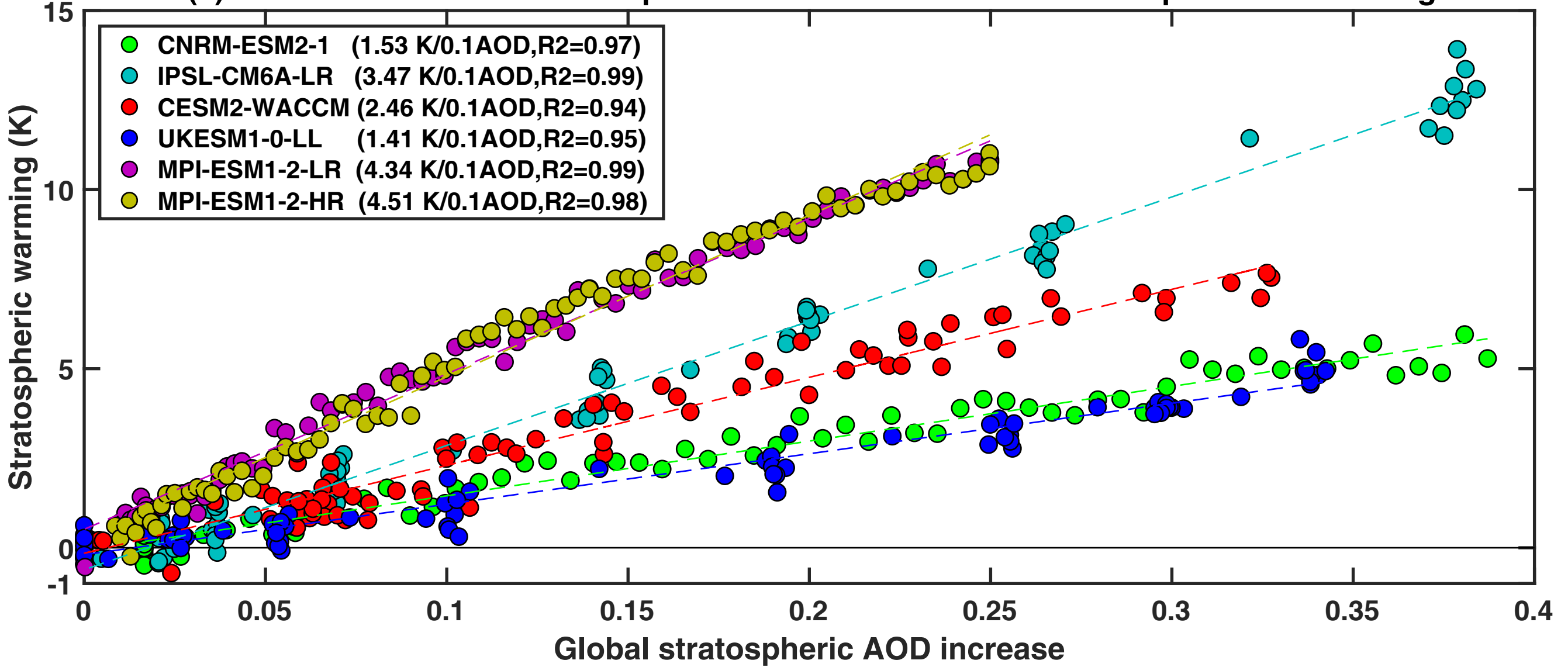
(c) Correlation between stratospheric aerosol increase and stratospheric air warming
