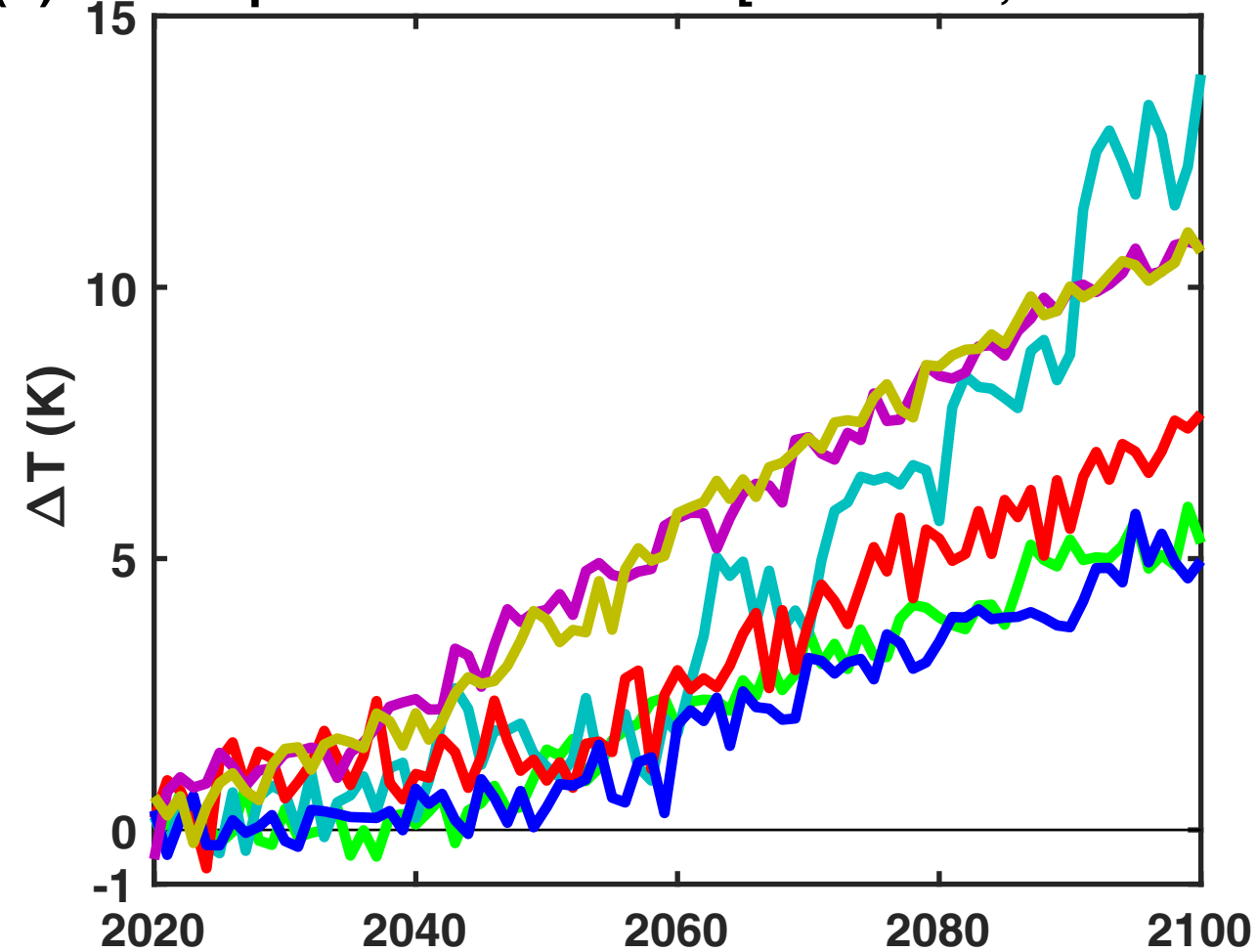
(b) Air temperature anomalies [20°N-20°S, 30-100 hPa]
