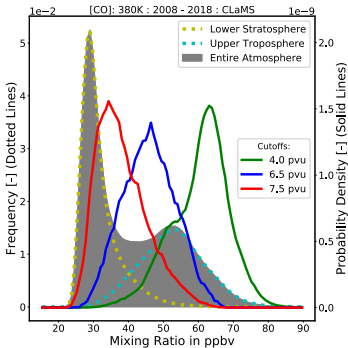
(a) CO
