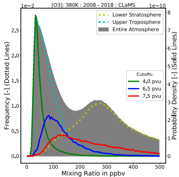
(c) O 3
