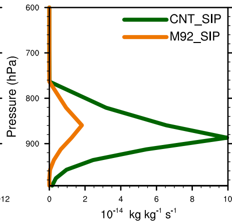
(f) graupel related IIC
