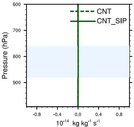
(e) Accumulation dust
