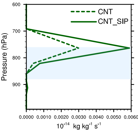
(f) Coarse dust
