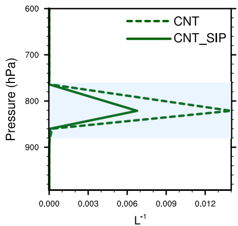
(g) Cloud droplet number
