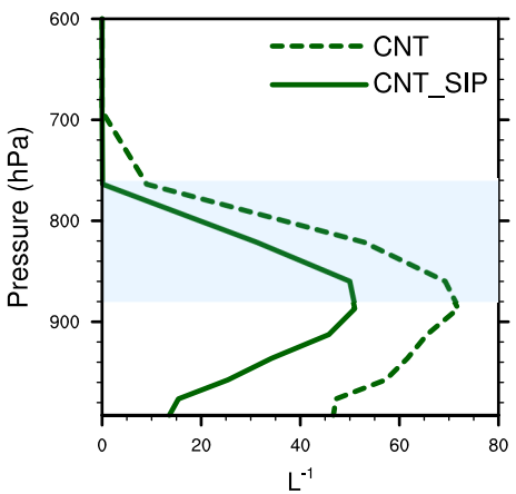
(h) Accrete cloud water by snow
