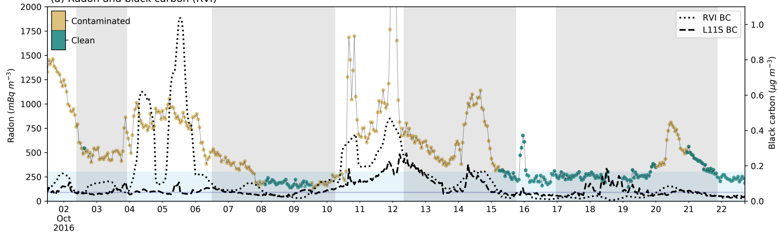
(a) Radon and black carbon (RVI)
