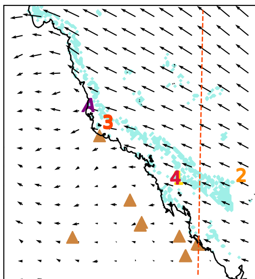
(b) Surface wind (L11SCR)
