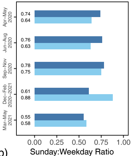
Pandora by Season
