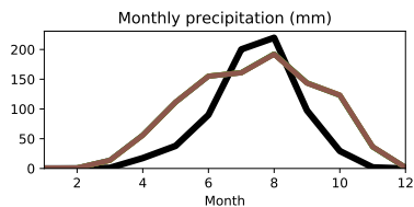
(c) Katibougou (12.93°N, 7.53°W)
