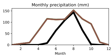
(b) Banizoumbou (13.52°N, 2.47°E)
