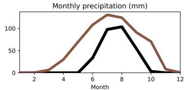
(a) Agoufou (15.34°N, 1.48°W)
