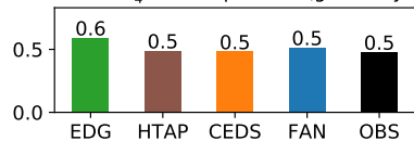
EANET: NH 4 + wet deposition (gN m -2 yr -1 )
