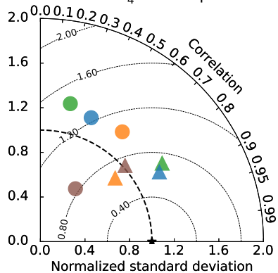
EANET: NH 4 + wet deposition (gN m -2 yr -1 )
