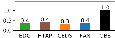
AMON: \text{NH}_3 ( \mu\text{gN m}^{-3} )
