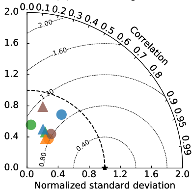
AMON: \text{NH}_3 ( \mu\text{gN m}^{-3} )
