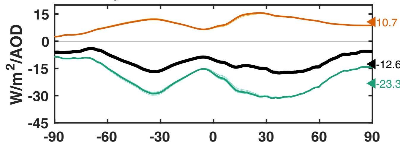
(c) \Delta F_d normalized to AOD [2081-2100]
