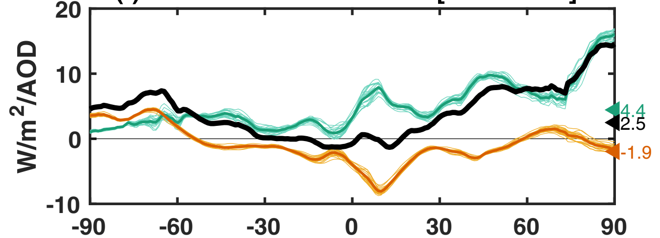
(f) \Delta C normalized to AOD [2081-2100]
