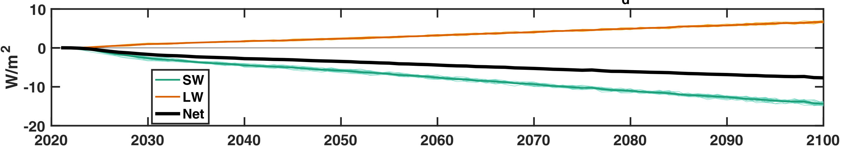
(b) \Delta F_d normalized to AOD [2026-2035]
