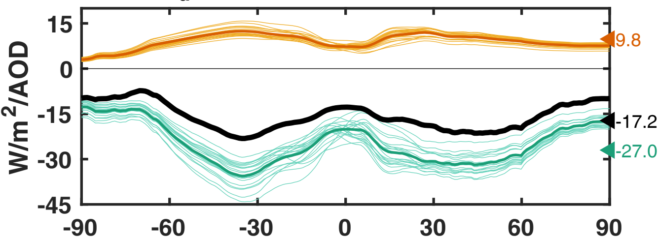
(b) \Delta F_d normalized to AOD [2026-2035]
