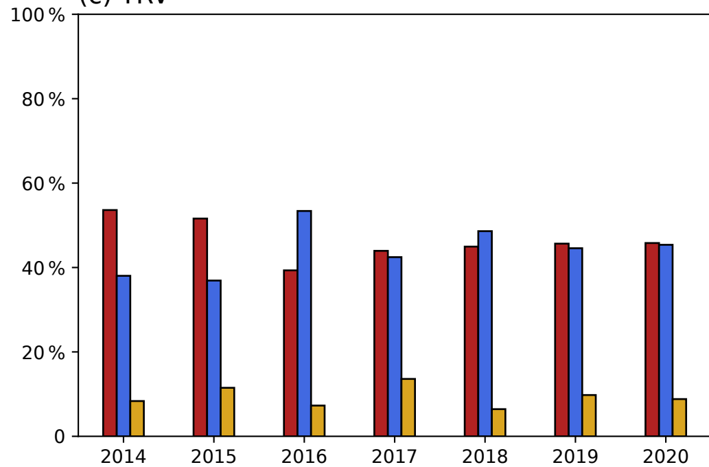
(c) YRV
