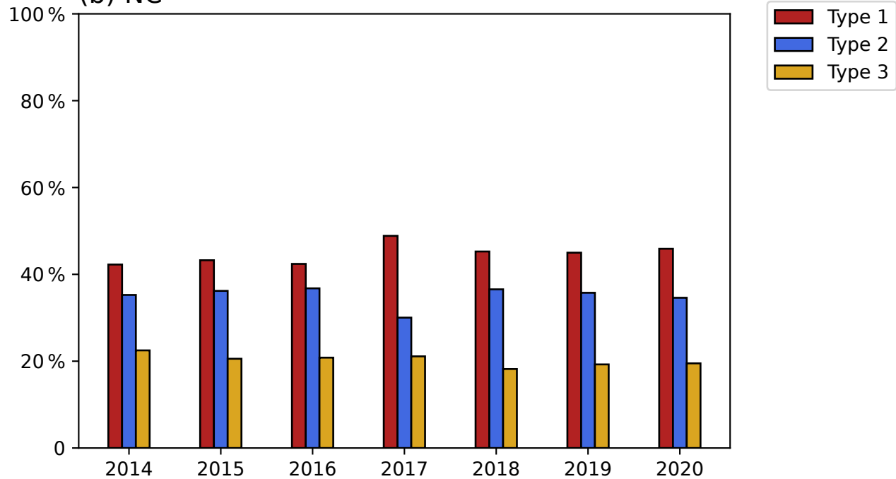
(b) NC
