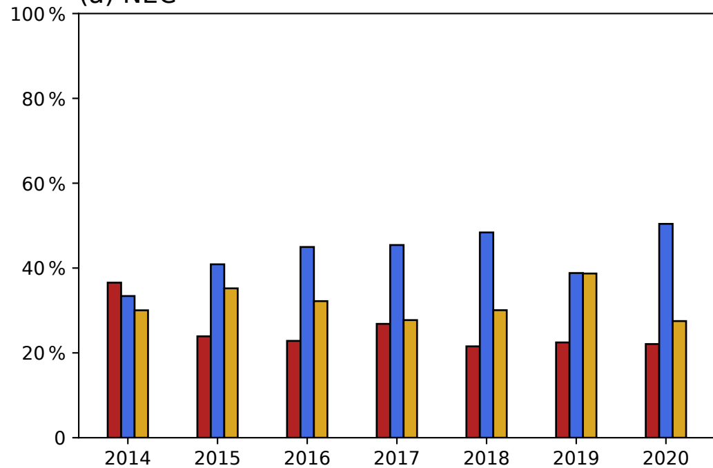
(a) NEC
