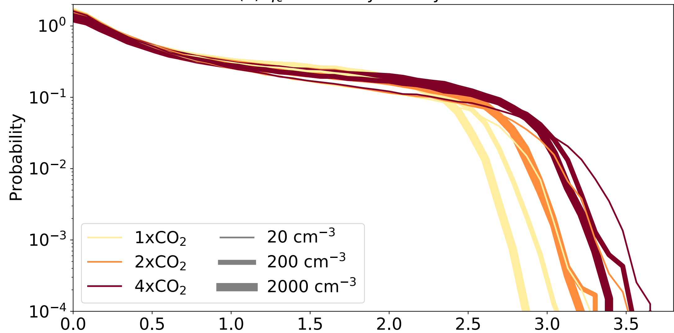
(a) q_c Probability density function
