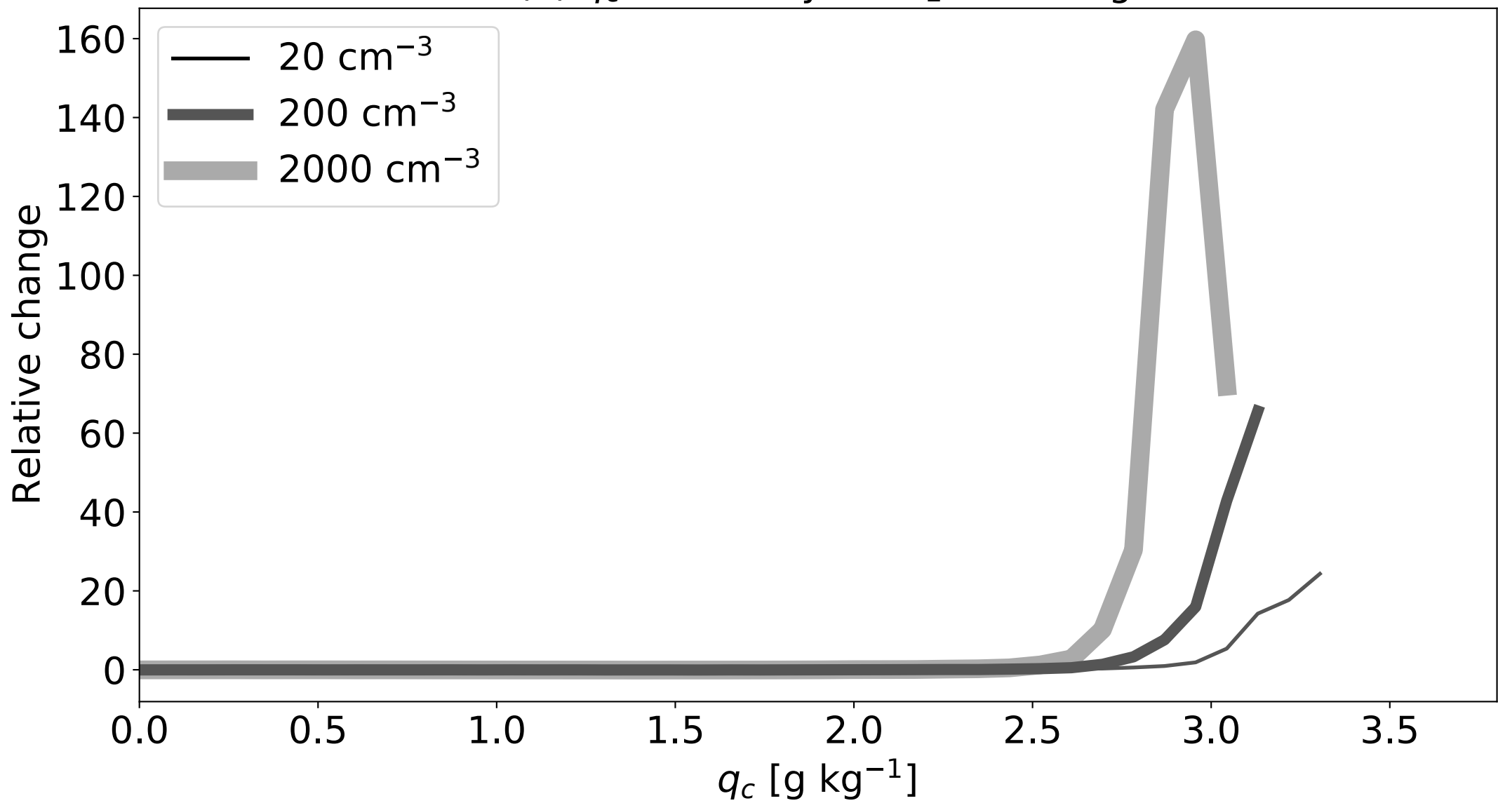
(b) q_c sensitivity to CO 2 doubling
