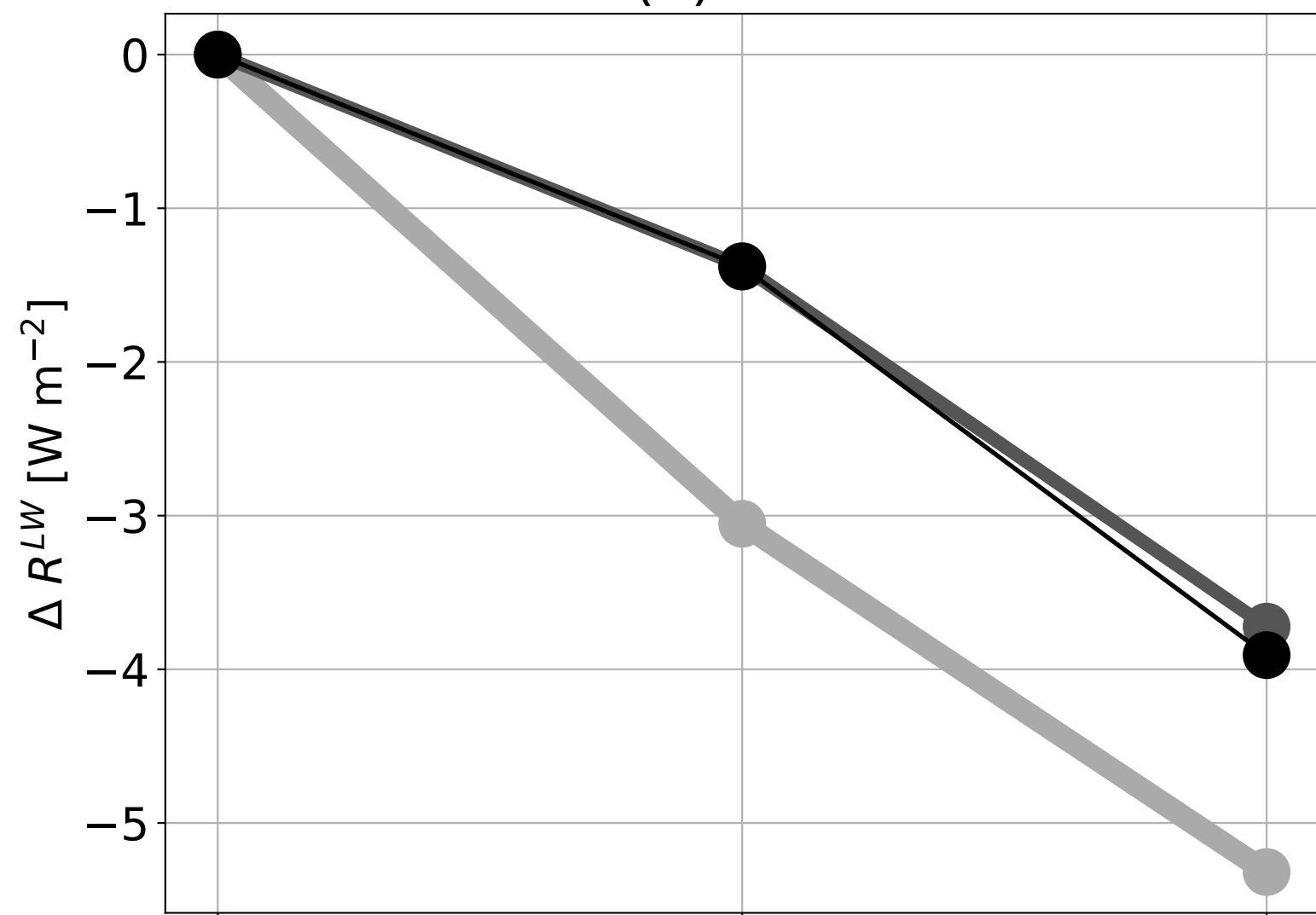
(b) R^{LW}
