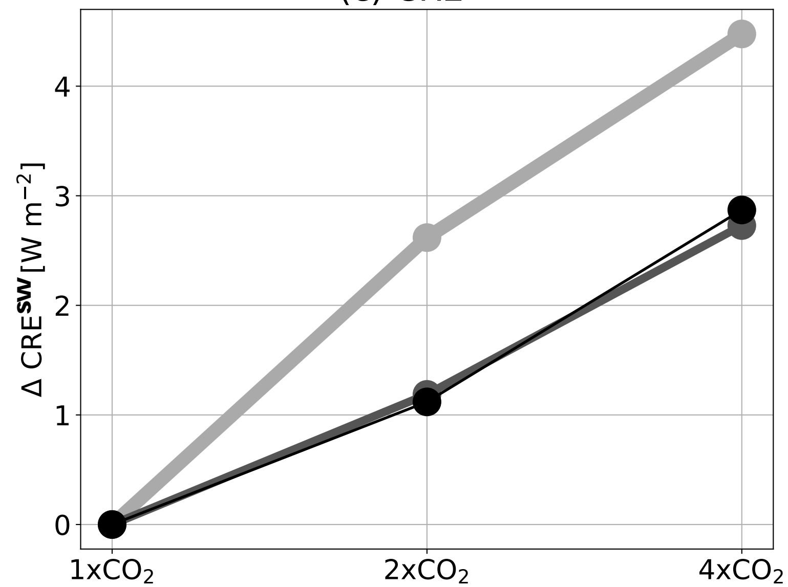
(c) CRE^{SW}
