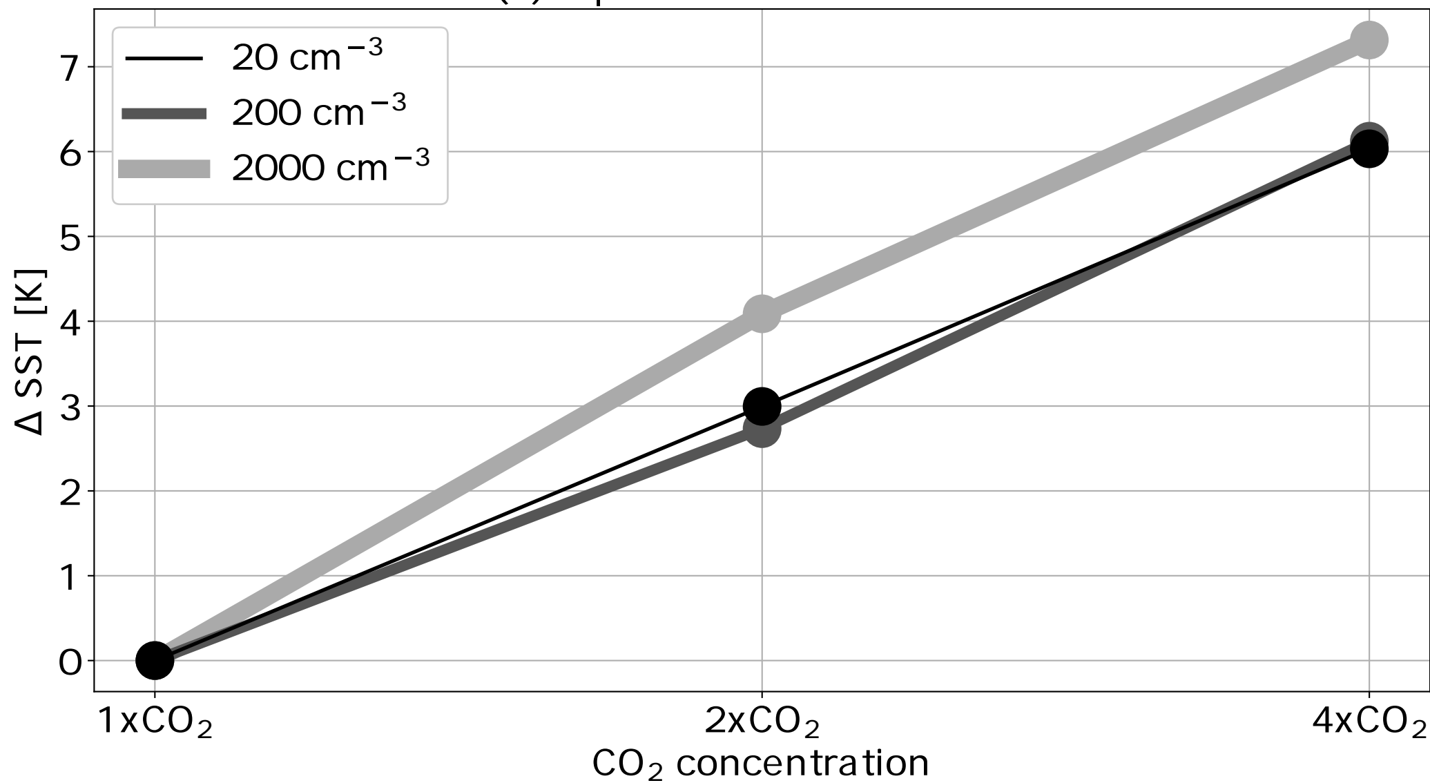
(b) Equilibrium SST difference
