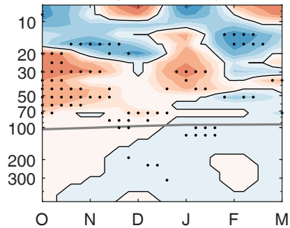
(c) dO3dt, 20°S-20°N, Niña
