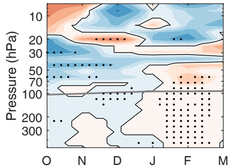
(a) dO3dt, 20°S-20°N, EP
