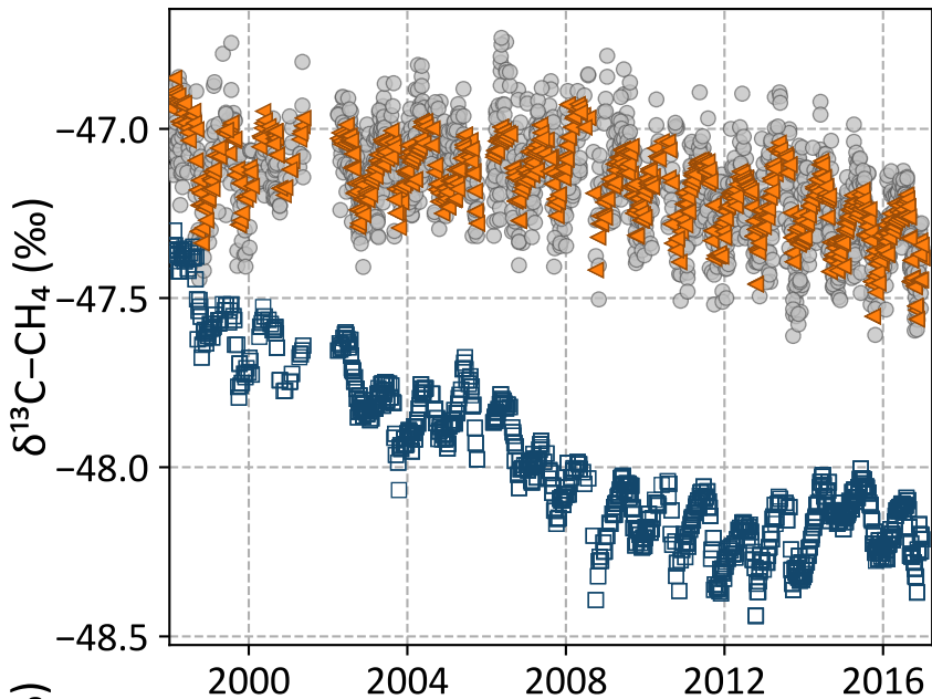
Mauna Loa, Hawaii (NOAA, United States)
