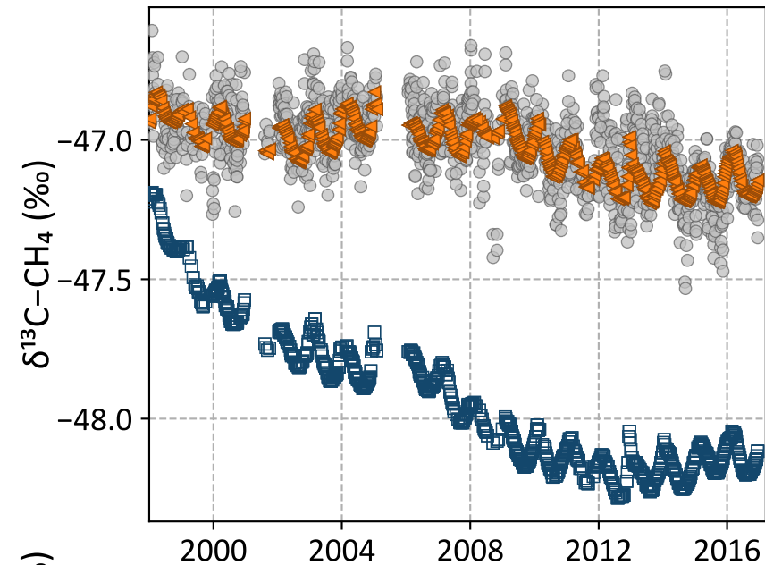
South Pole, Antarctica (NOAA, United States)
