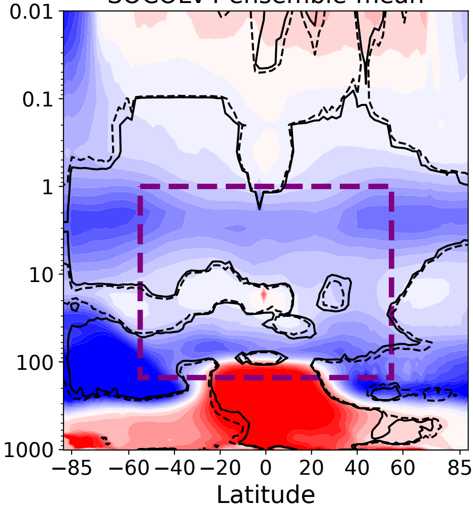
SOCOLv4 ensemble-mean
