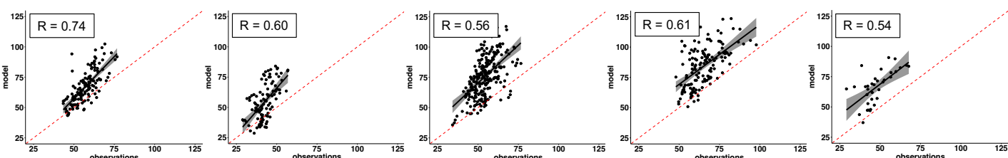
Cluster 1 - HMO
