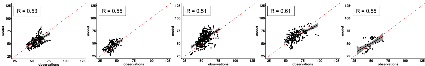
Cluster 1 - HMO
