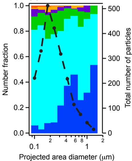
(b) Observed BLSN
