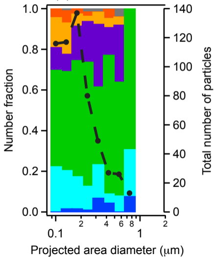
(a) Moderate wind
