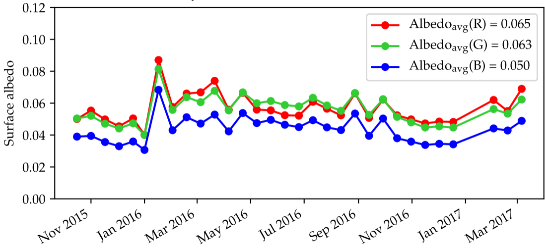
MODIS white sky albedo (MCD43A3) for HaloCam RAW RGB channels
