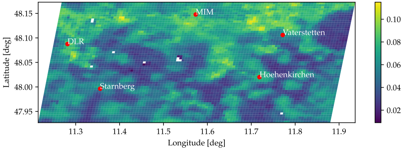
MODIS MCD43A3 white sky albedo, 555 nm, 2015-09-19
